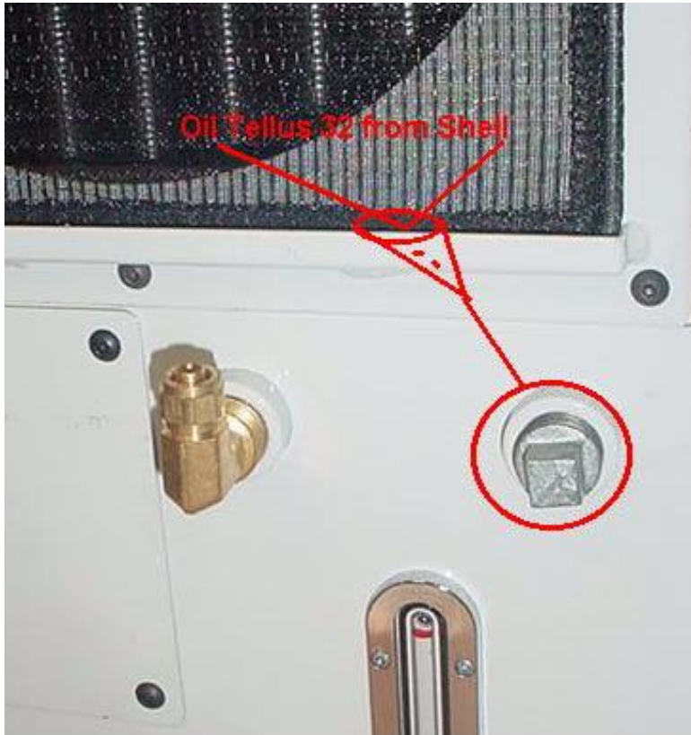
Oil spindle chiller on the machine
